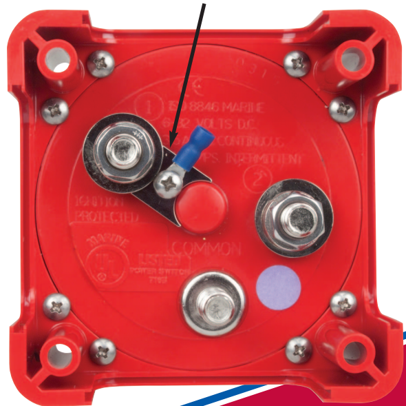
Accessory Tap shown installed with wire terminal (not included)
